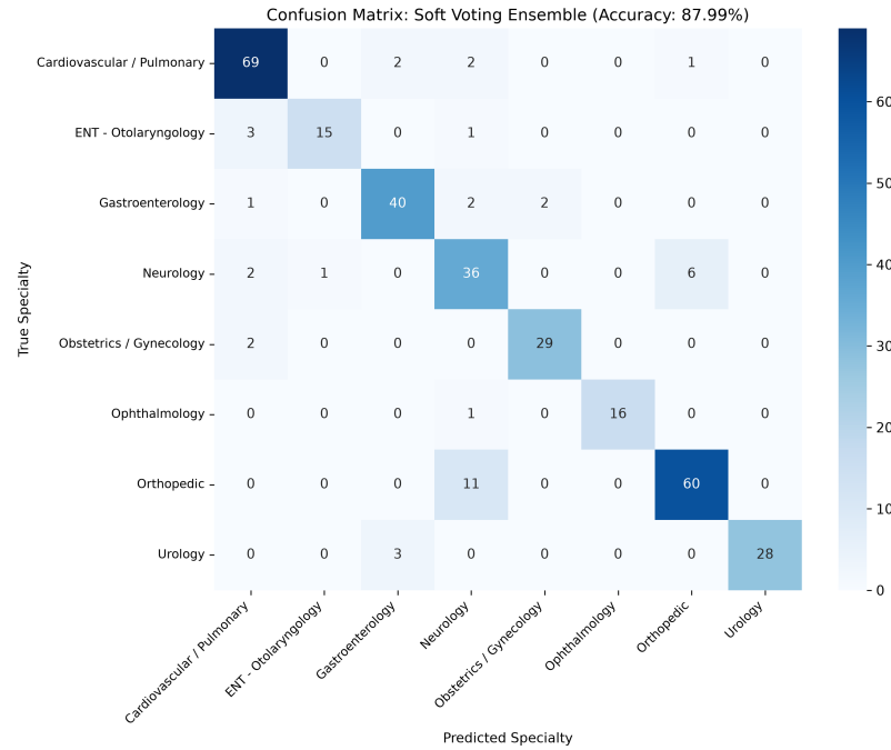
Figure 15: Confusion Matrix of the Soft Voting Ensemble across 8 Clinical Specialties on the Held-Out Test Set
