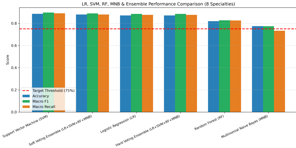
Figure 14: Model Performance Comparison across Accuracy, Macro F1, and Macro Recall against the 75% Target Threshold
